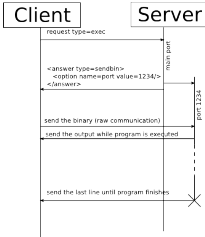
Figure 14.1: TASTE Daemon execution protocol overview
