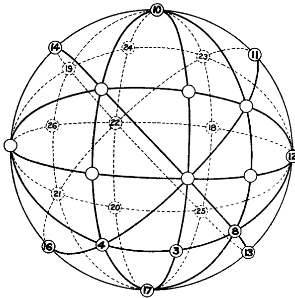
Figure 4.34 Magic sphere.
