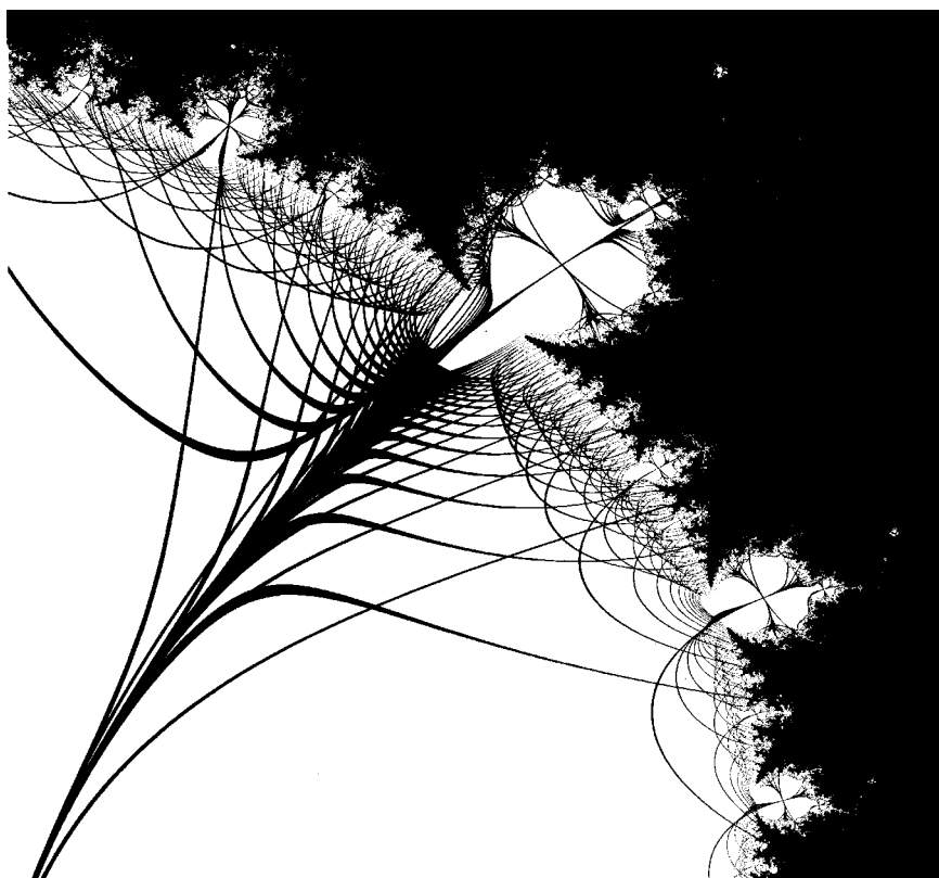
Figure 4.59 Mandelbrot stalks.
