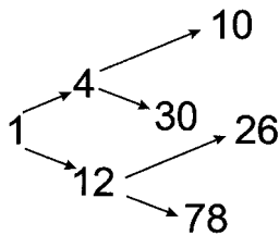
Figure 2.2 Grasshopper sequences.
