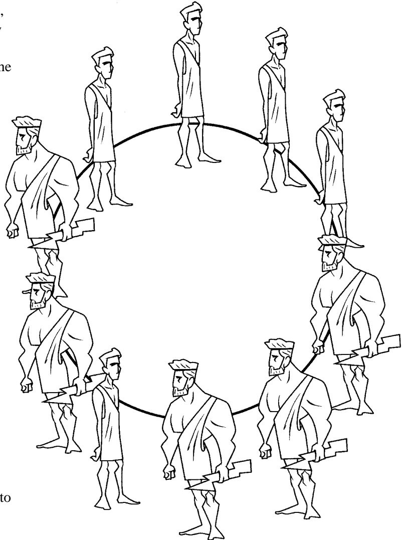
Figure 5.9 Plato's choice.
