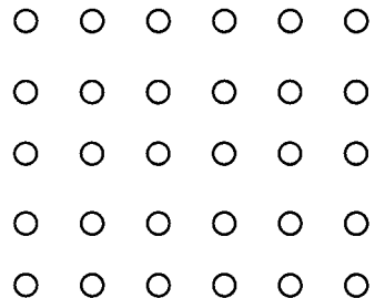
Figure 4.20 Mystery triangles.
