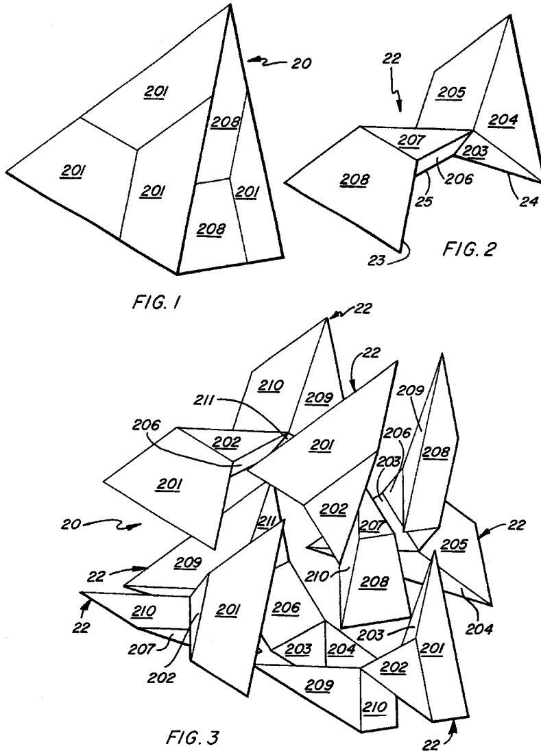
Figure 4.66 Platonic patent.
