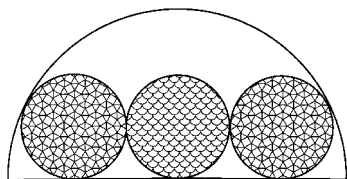
Figure 2.4 Golden circles.
