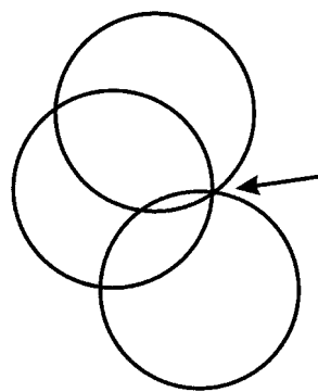
Figure 4.14 Circle crossing.
