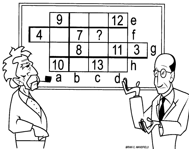
Figure 4.10 Mondrian puzzle.
